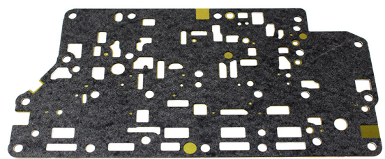
8F24 Bonded V/Body Plate Lower Part No. 106.VB.31
