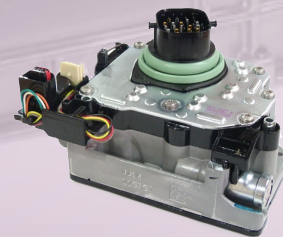
62TE Switch Pressure Transducer Part No. 72.SW.11 (Located on Valve body)
